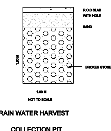
RAIN WATER HARVEST COLLECTION PIT.
