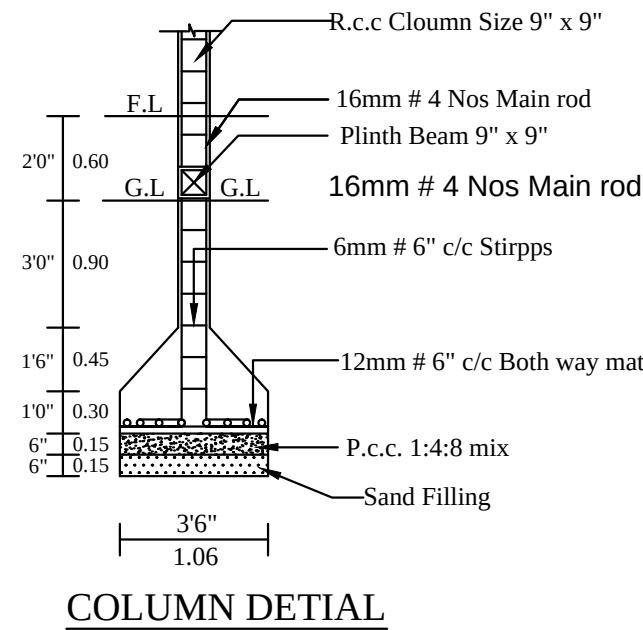
COLUMN DETIAL
