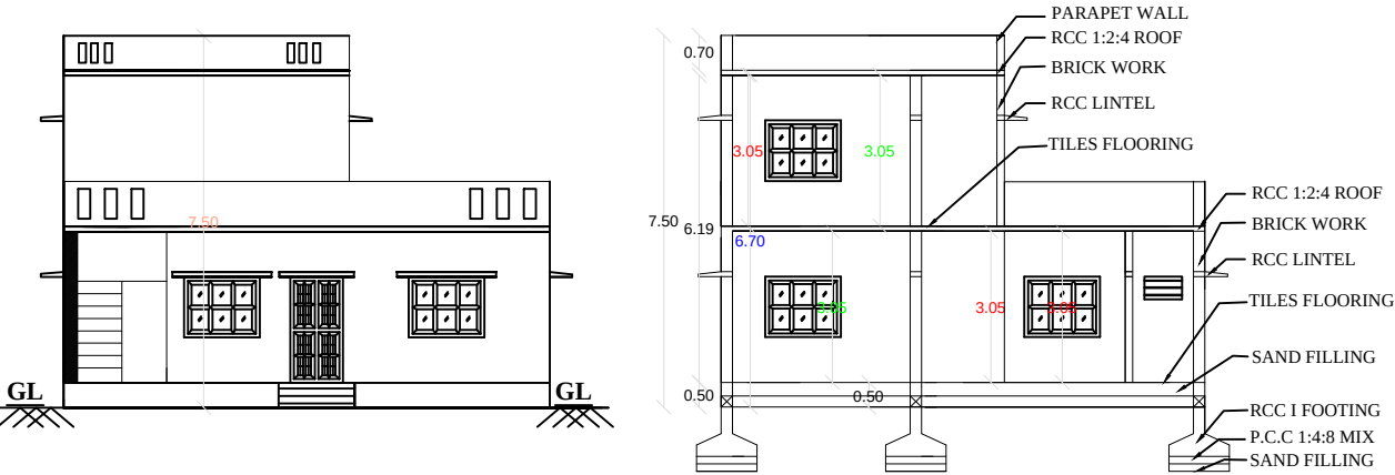
FRONT ELEVATION
