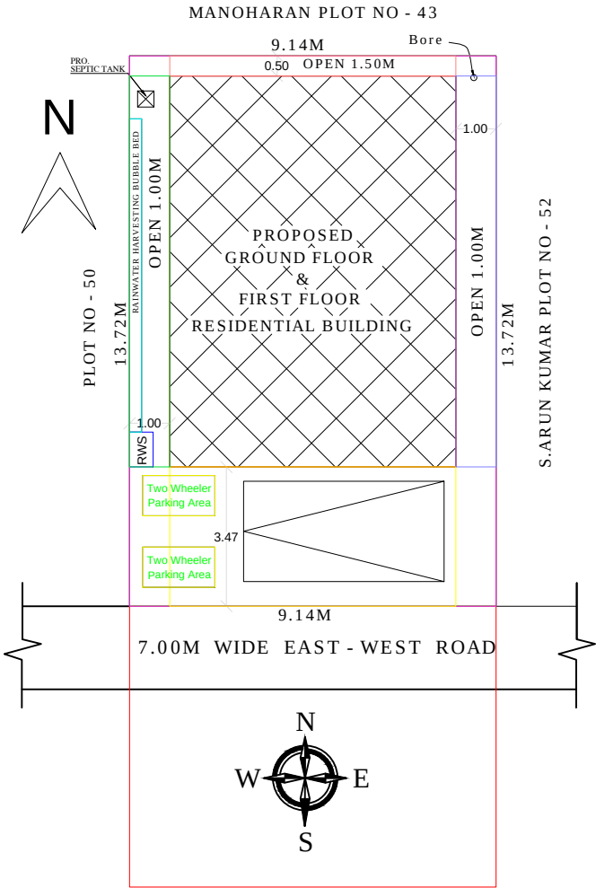
SITE PLAN (SCALE 1:1)
