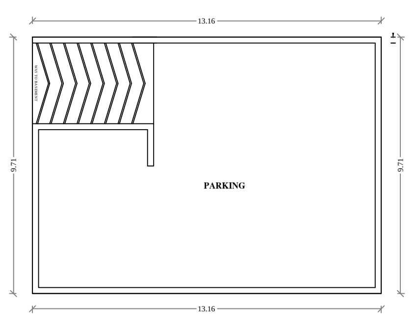
STILT FLOOR PLAN
