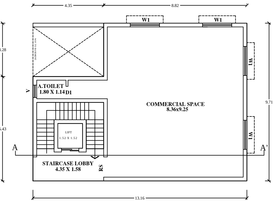
EXG. FIRST FLOOR PLAN
