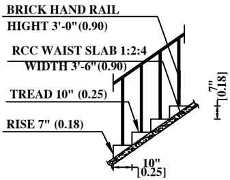
STAIRCASE DETAIL SCALE 1:50
