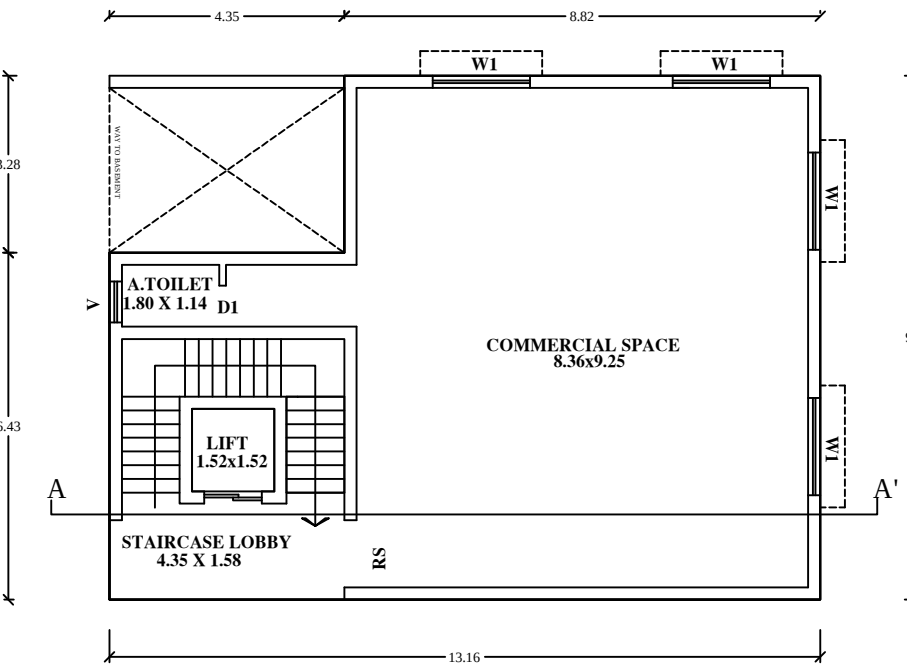
EXG. GROUND FLOOR PLAN
