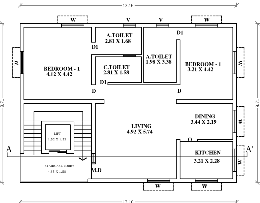
PRO. SECOND FLOOR
