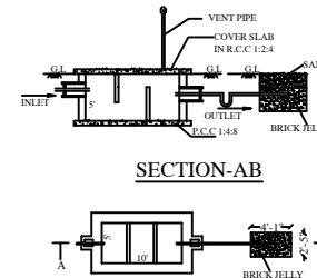
SEPTIC TANK & DISPERSION TRENCH DETAILS
