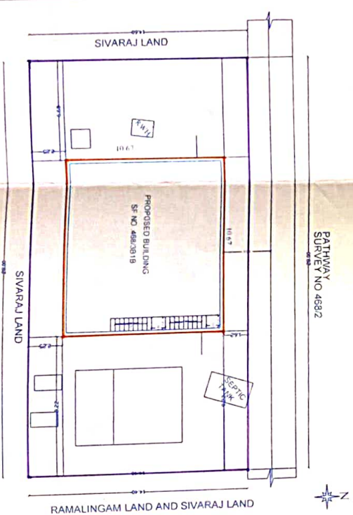
KEY PLAN
