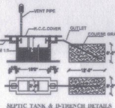
SEPTIC TANK & D-TURNCH DETAILS
