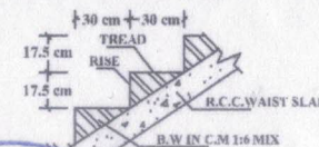
SECTION OF STAIRCASE
