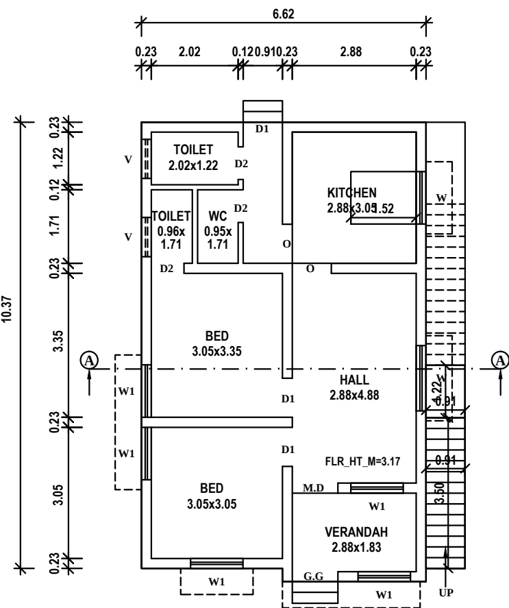
EXG.GROUND FLOOR PLAN
