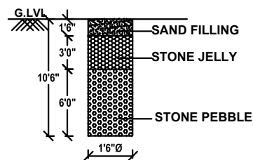
RAIN WATER HARVESTING PIT (NOT TO SCALE)
