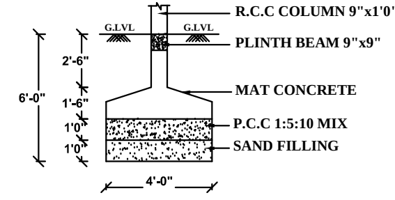
COLUMN FOUNDATION (NOT TO SCALE)
