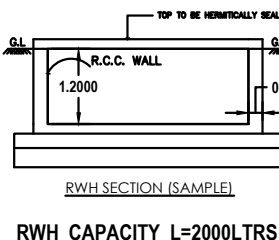
RWH CAPACITY_L=2000LTRS
