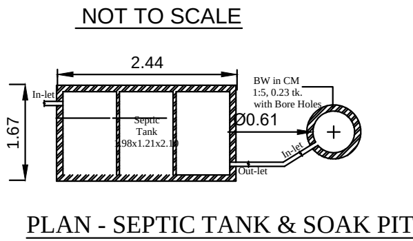
PLAN - SEPTIC TANK & SOAK PIT
