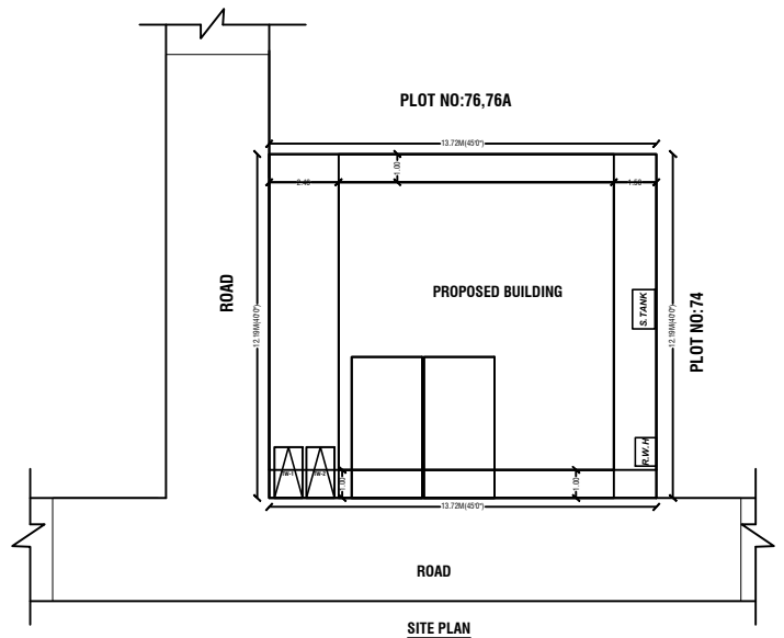
SITE PLAN
