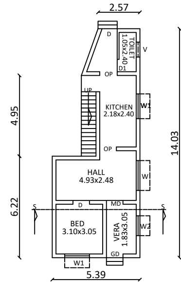
EXG) GROUND FLOOR PLAN
