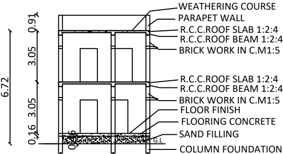
SECTION- SS
