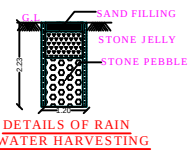
DETAILS OF RAIN WATER HARVESTING
