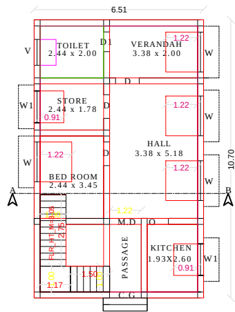
PRO.GROUND FLOOR PLAN (SOUTH FACING)
