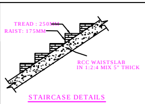
STAIRCASE DETAILS
