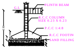
TYPICAL SECTION OF R.C.C COLOUMN FOOTING
