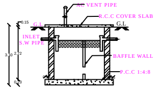
SEPTIC TANK DETAILS
