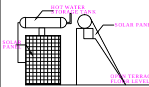
PLAN SIDE ELEVATION SOLAR SYSTEM DETAILS
