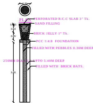
PERCOLATION PIT SECTION OF RAIN WATER
