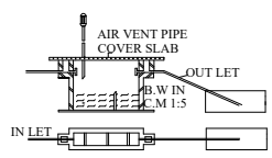
DETAILS OF SEPTIC TANK & D-TRENCH
