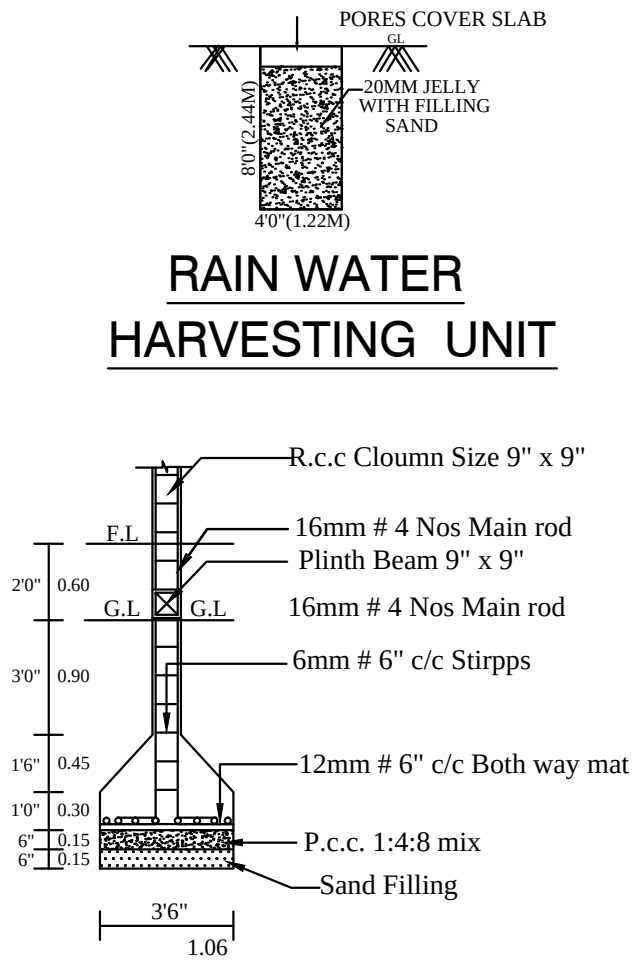
COLUMN DETIAL
