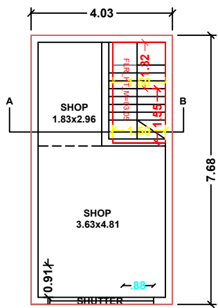
EXISTING GROUND FLOOR
