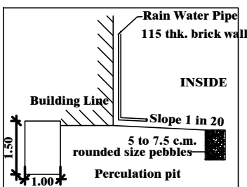
RAIN WATER PIPE DETAIL
