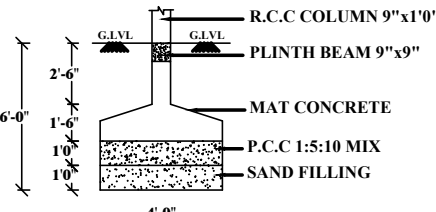
COLUMN FOUNDATION (NOT TO SCALE)
