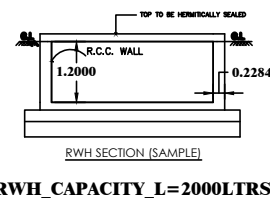
RWH_CAPACITY_L=2000LTRS
