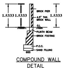
COMPOUND WALL DETAIL
