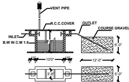
SEPTIC TANK & D-TRENCH DETAILS (NOT TO SCALE)
