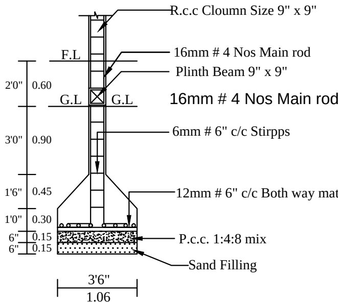
COLUMN DETIAL
