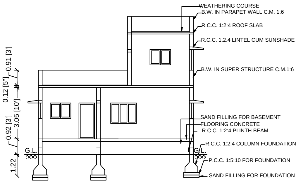
SECTION - "AB"
