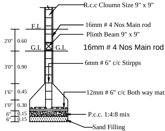
COLUMN DETIAL
