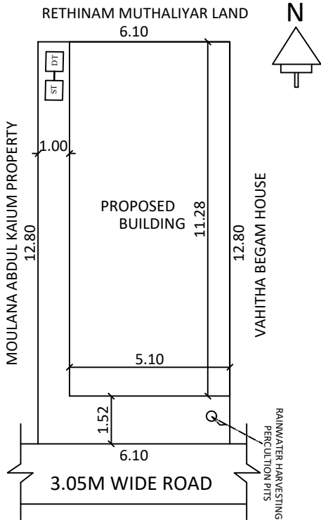
SITE PLAN
