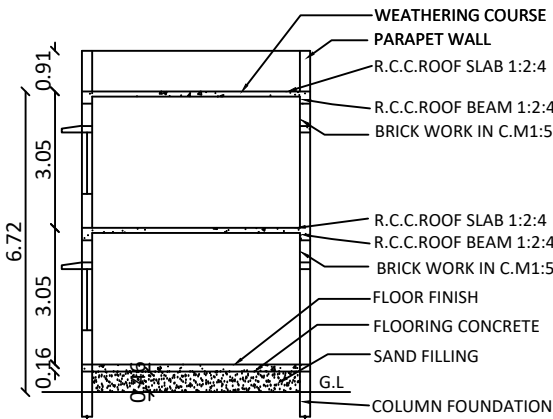
SECTION ON GG
