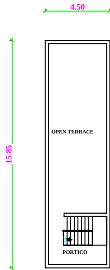
TERRACE FLOOR
