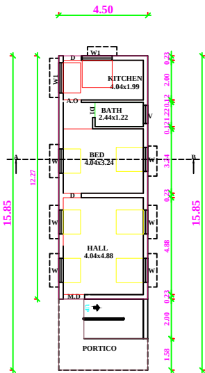
FLOOR-GROUND
