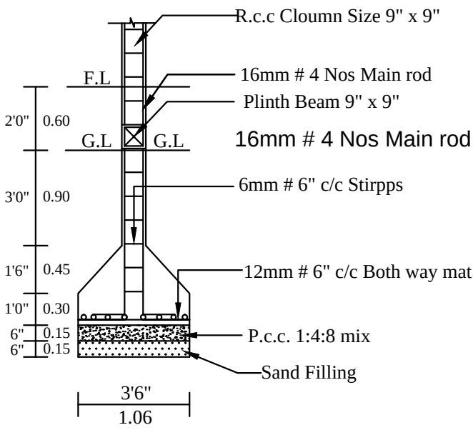
COLUMN DETIAL
