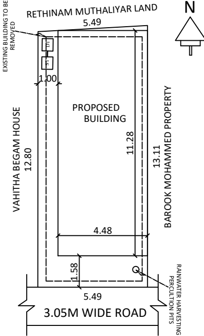
SITE PLAN
