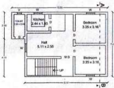
FLOOR PLAN
