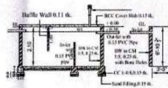
SECTION - SEPTIC TANK & SOAK PIT
