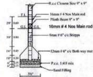
COLUMN DETAIL
