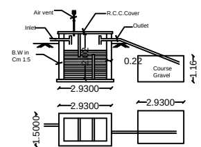
SEPTIC TANK & D-TRENCH DETAILS
