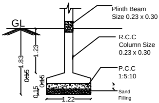
FOUNDATION DETAILS
