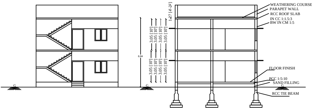
FRONT ELEVATION
