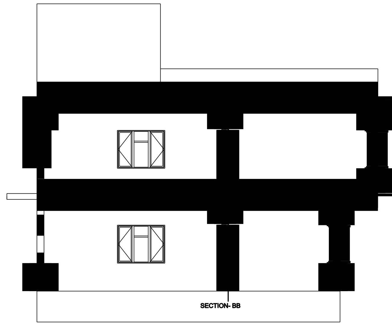
SECTION- BB
