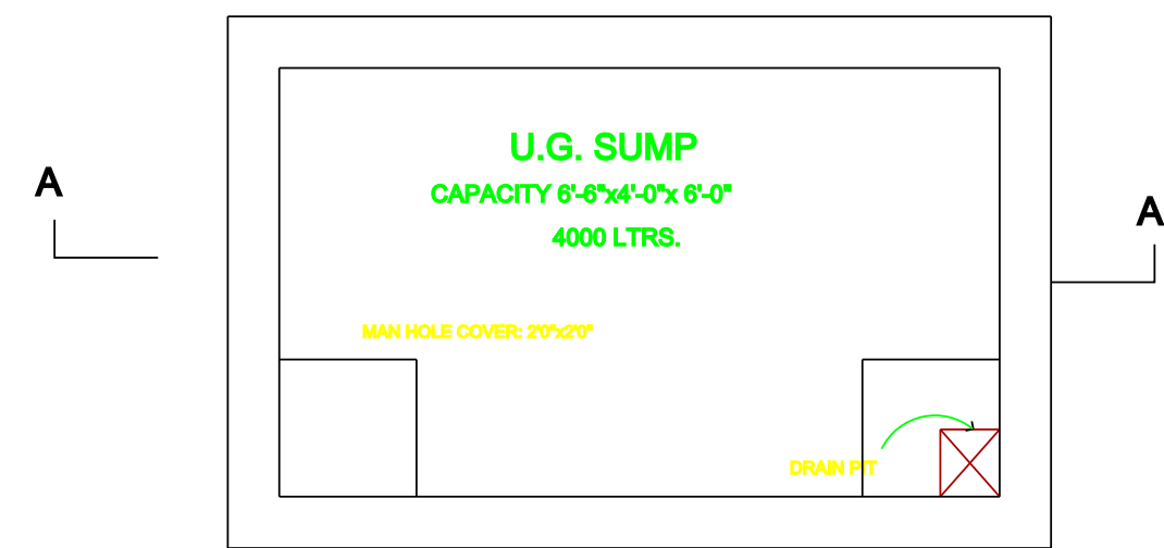
SUMP DETAIL
