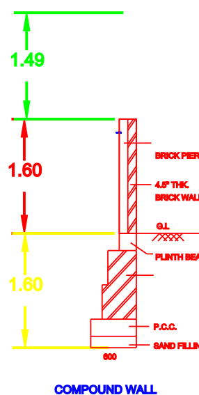
COMPOUND WALL
