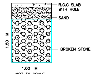
RAIN WATER HARVEST COLLECTION PIT.
