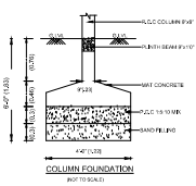
COLUMN FOUNDATION (NOT TO SCALE)
