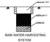
RAIN WATER HARVESTING SYSTEM (NOT TO SCALE)
