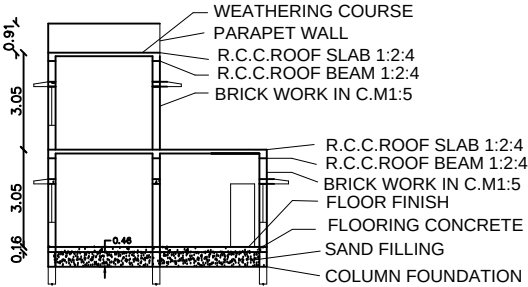
SECTION- SS
