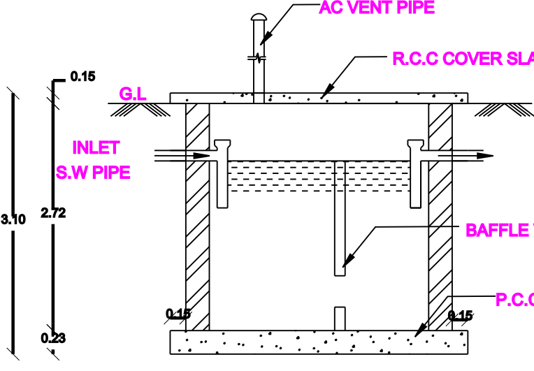
SAEPTIC TANK DETAILS
