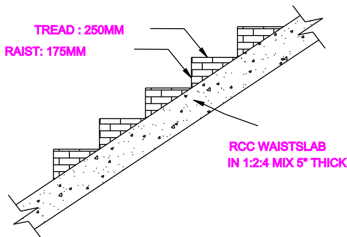
STAIRCASE DETAILS
