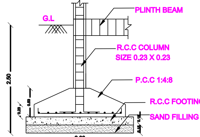
TYPICAL SECTION OF R.C.C COLOUMN FOOTING
