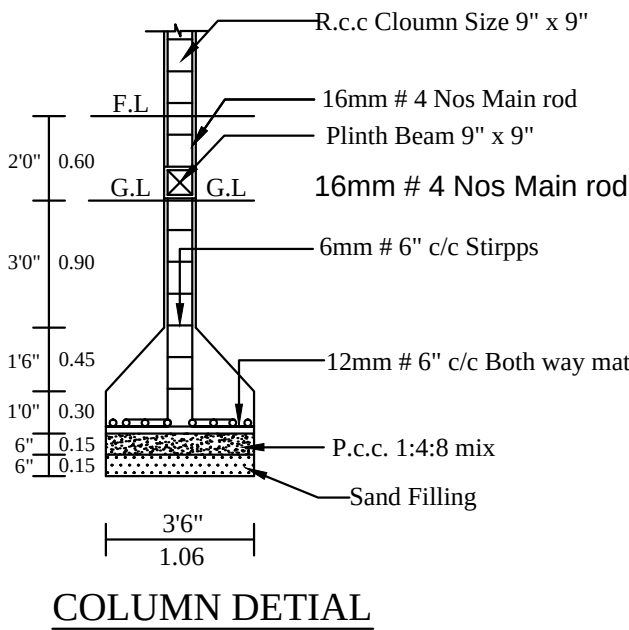
COLUMN DETIAL
