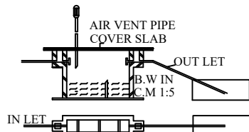
DETAILS OF SEPTIC TANK & D-TRENCE
