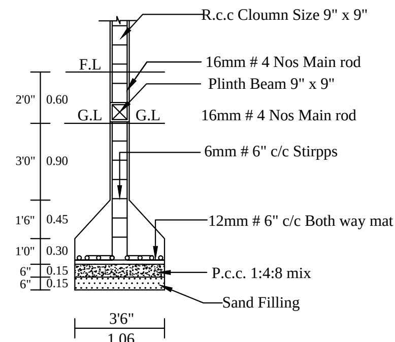
COLUMN DETIAL
