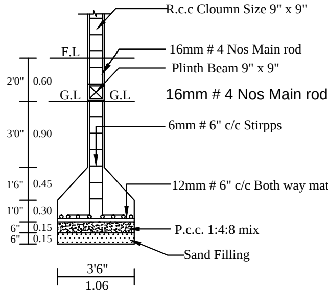
COLUMN DETIAL
