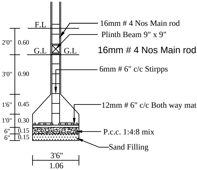
COLUMN DETIAL
