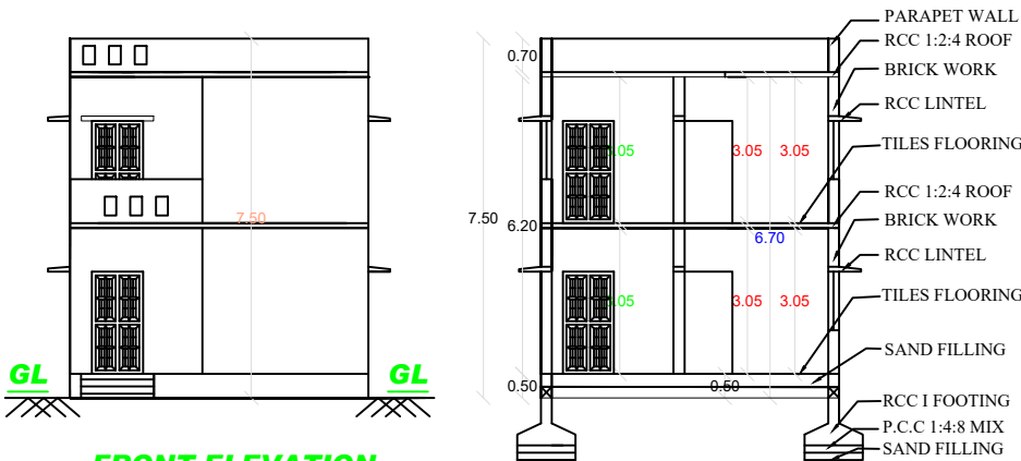
FRONT ELEVATION
