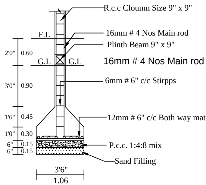
COLUMN DETIAL
