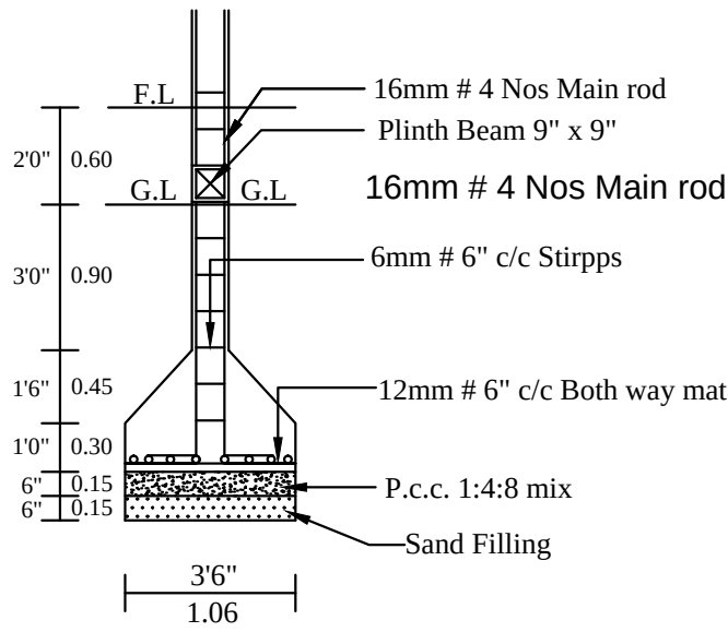
COLUMN DETIAL
