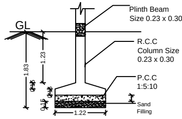
FOUNDATION DETAILS
