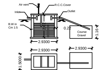
SEPTIC TANK & D-TRENCH DETAILS
