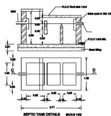
SEPTIC TANK DETAILS (SCALE: 1:100)
