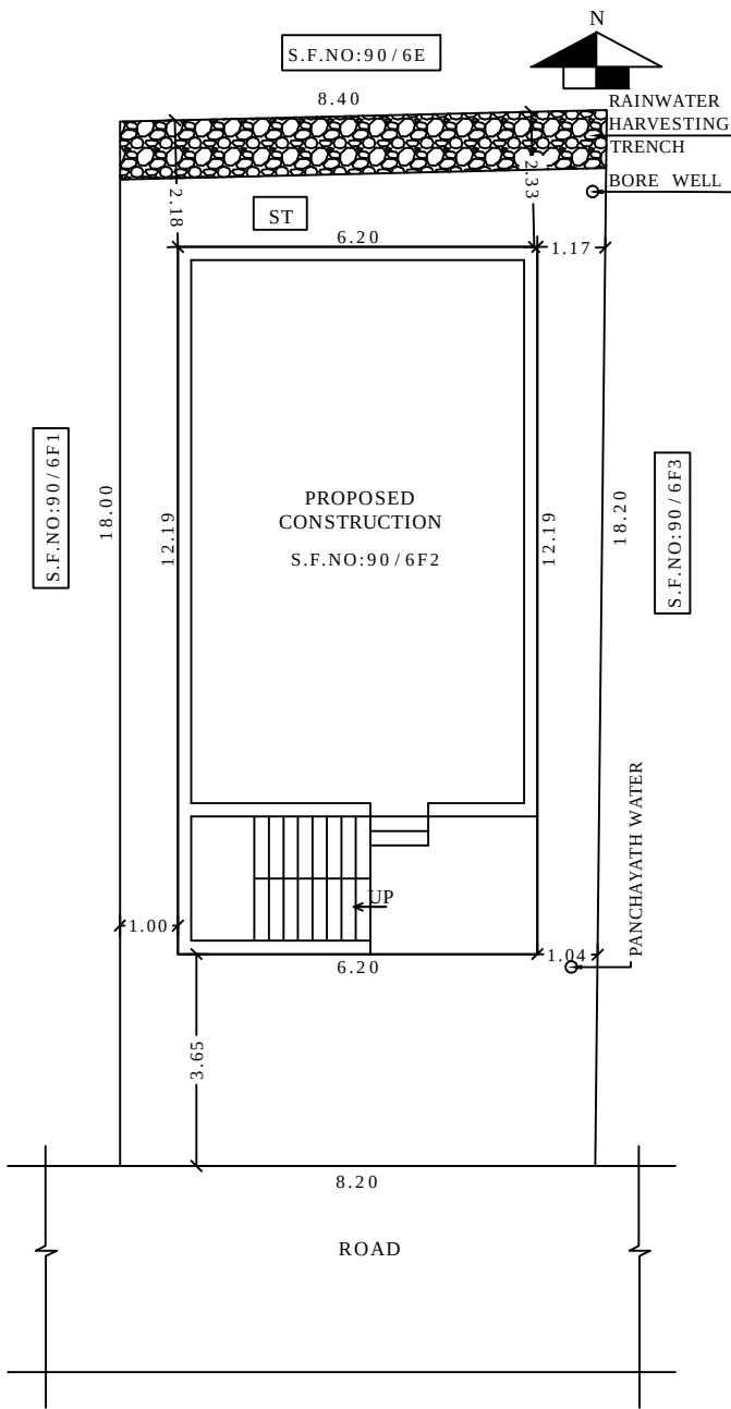
SITE PLAN
