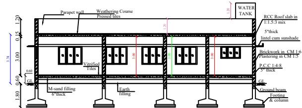
SECTION X-X
