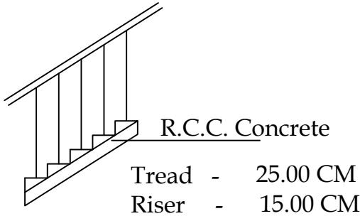
Staircase details
