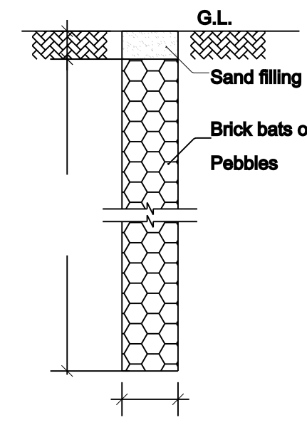
Percolation Pit
