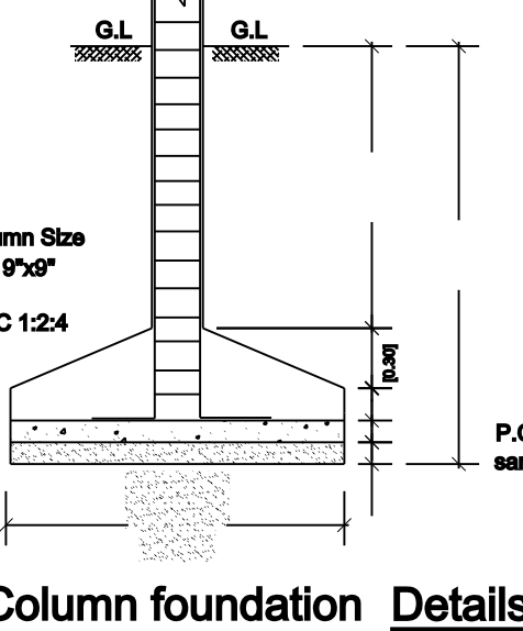
Column foundation Details
