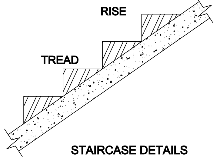
STAIRCASE DETAILS (SCALE = 1 : 50)
