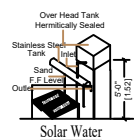
Solar Water Heating System
