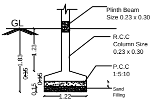
FOUNDATION DETAILS
