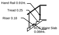
STAIRCASE DETAILS (Not to Scale)
