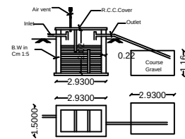
SEPTIC TANK & D-TRENCH DETAILS
