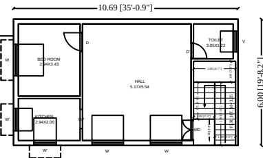
FLOOR 1
