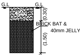
RAIN WATER HARVESTING SYSTEM
