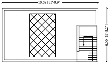
TERRACE PLAN
