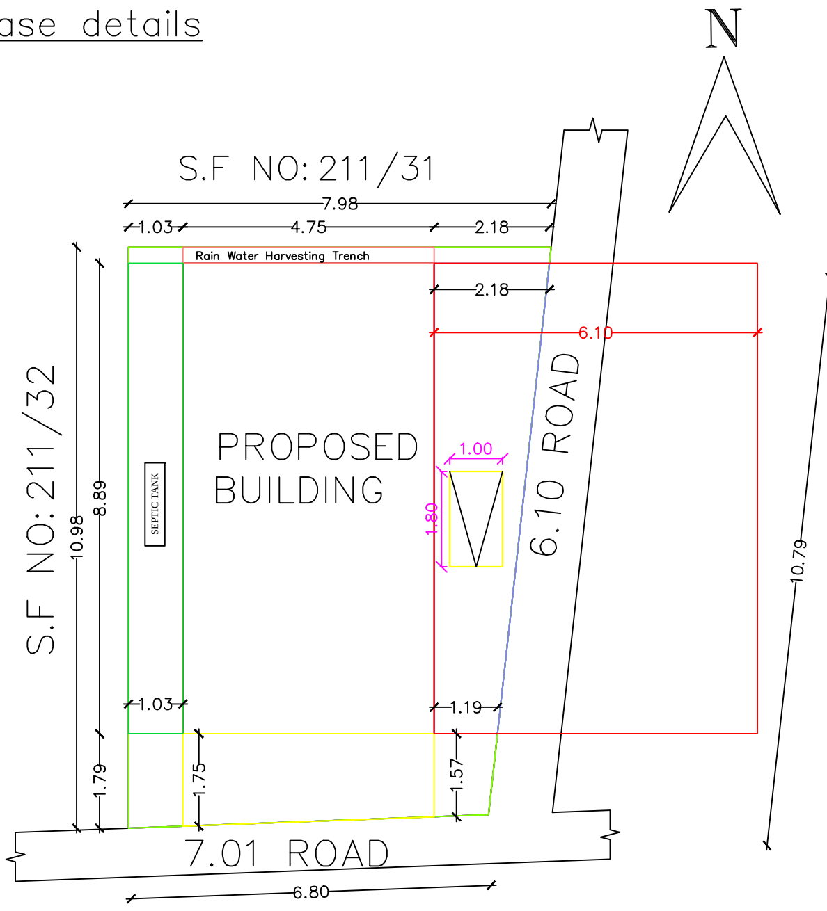
SITE PLAN
