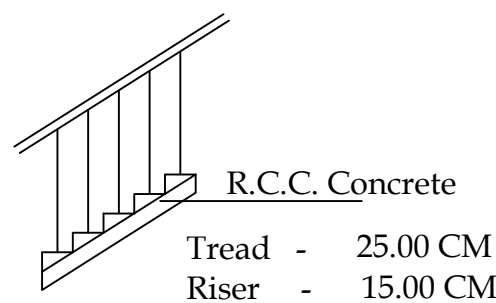
Staircase details
