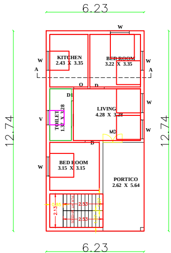
FLOOR- GROUND
