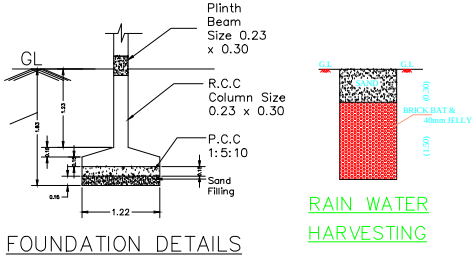
FOUNDATION DETAILS
