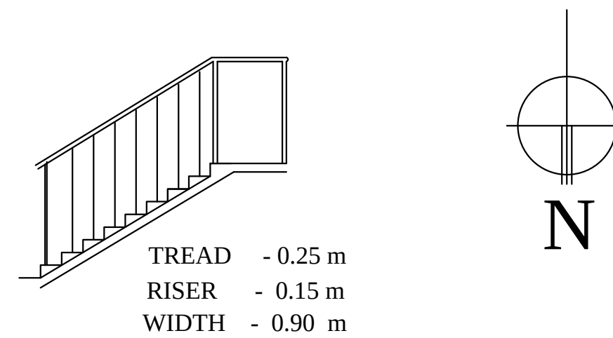
STAIRCASE DETAILS
