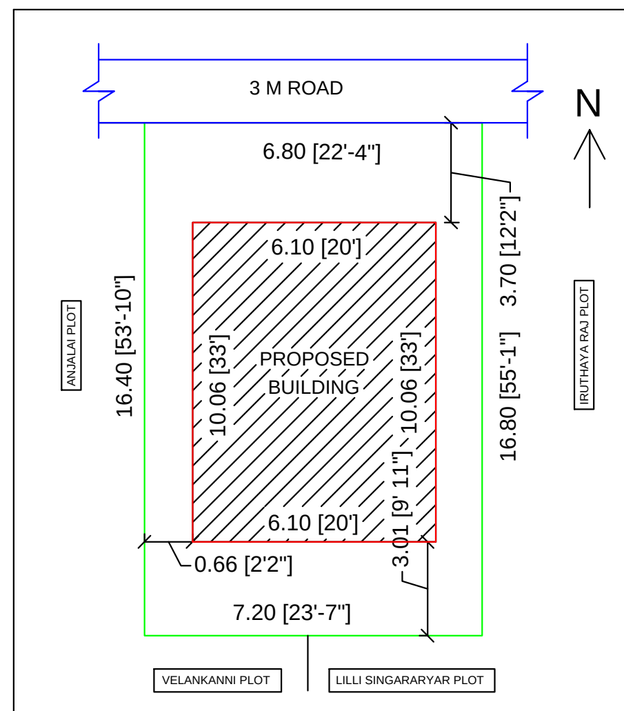
LOCATION PLAN
