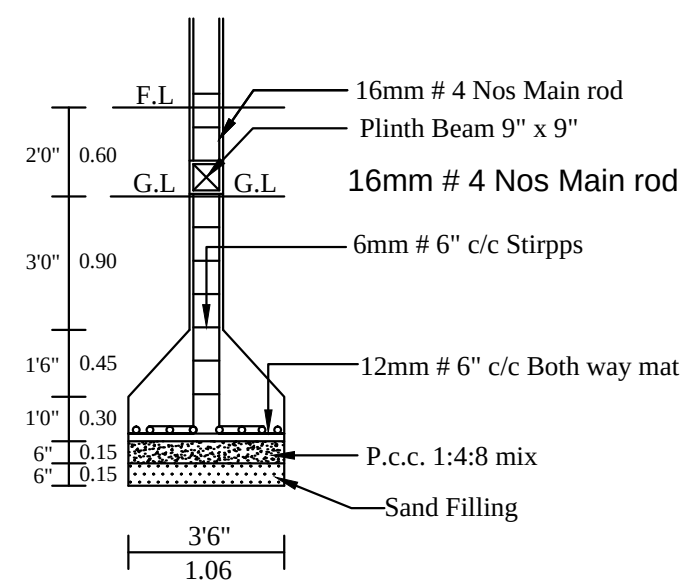
COLUMN DETIAL
