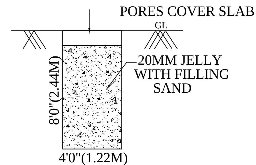
RAINWATER HARVESTING UNIT
