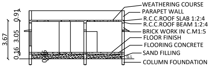
SECTION- SS
