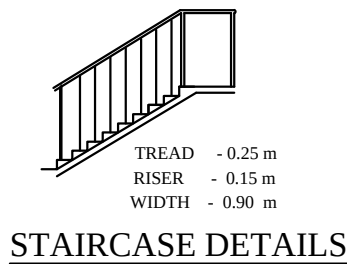
STAIRCASE DETAILS
