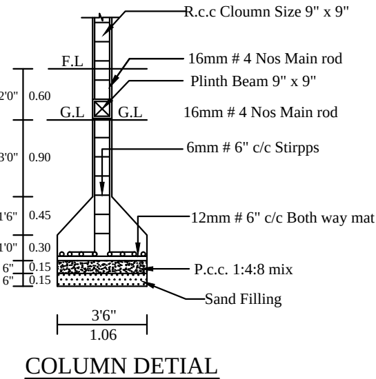
COLUMN DETIAL
