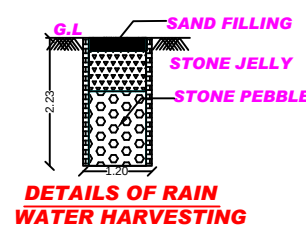
DETAILS OF RAIN WATER HARVESTING
