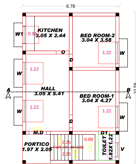
PRO.GROUND FLOOR PLAN (NORTH FACING)
