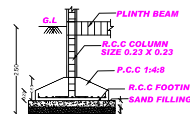
TYPICAL SECTION OF R.C.C COLOUMN FOOTING
